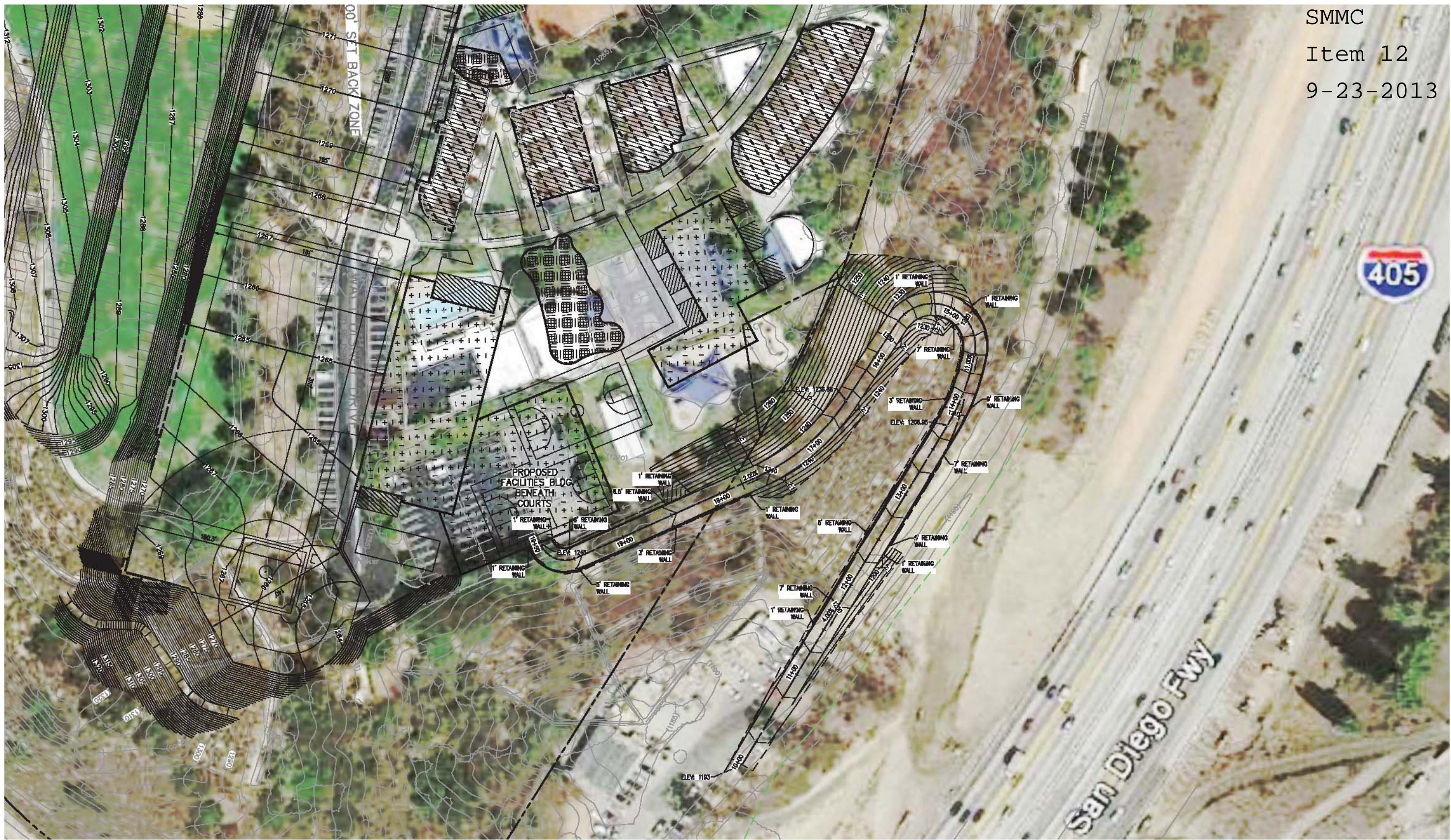
Figure A-4-3 Aerial View of the Proposed Secondary Access Road
